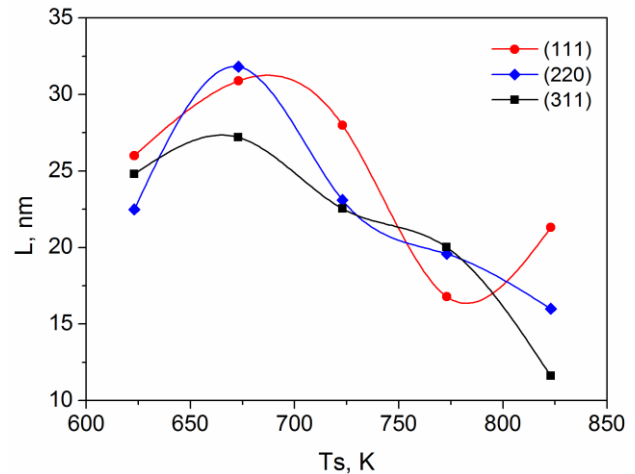
Fig. 5 – Dependence of CSR sizes ( L ) of \text{Cd}_x\text{Zn}_{1-x}\text{Te} films on substrate temperature. Values for the crystallographic directions [111], [220] and [311] are presented.
